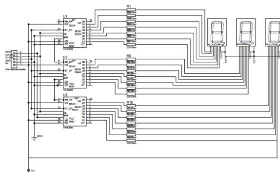
Gambar 5. Rangkaian Seven Segmen
