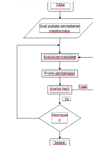
Gambar 2. Flowchart penelitian
