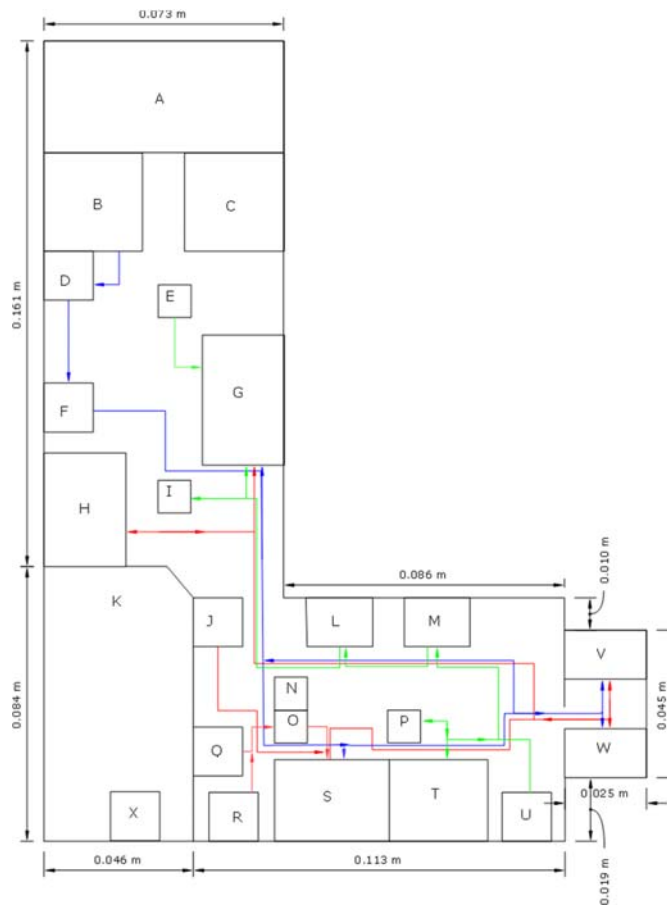
Gambar 3. Layout Awal
