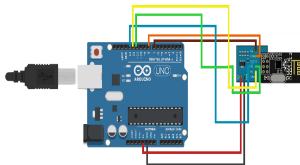
Gambar 3. Wiring Receiver
