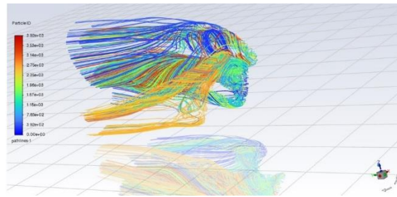
Gambar 7. Streamline FPP \phi 70 3 pitch
