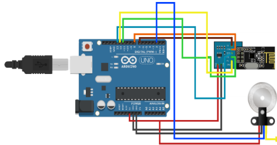
Gambar 4 Wiring Transmitter
