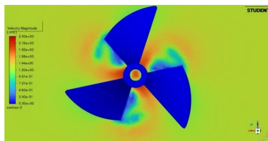
Gambar 6. Contour Velocity FPP \phi 70 3 pitch
