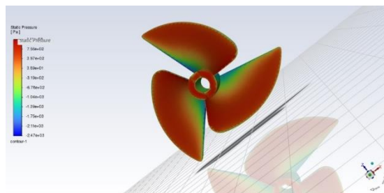
Gambar 5. Contour Pressure FPP \phi 70 3 pitch
