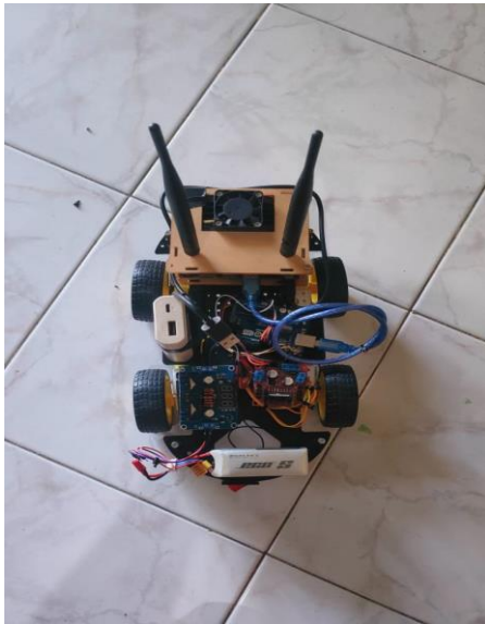
Gambar 2. Prototype robot mobil berbasis ROS
